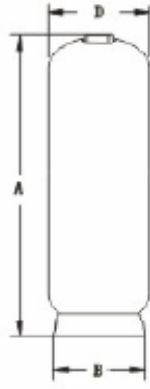
18"-36" Standard Base
